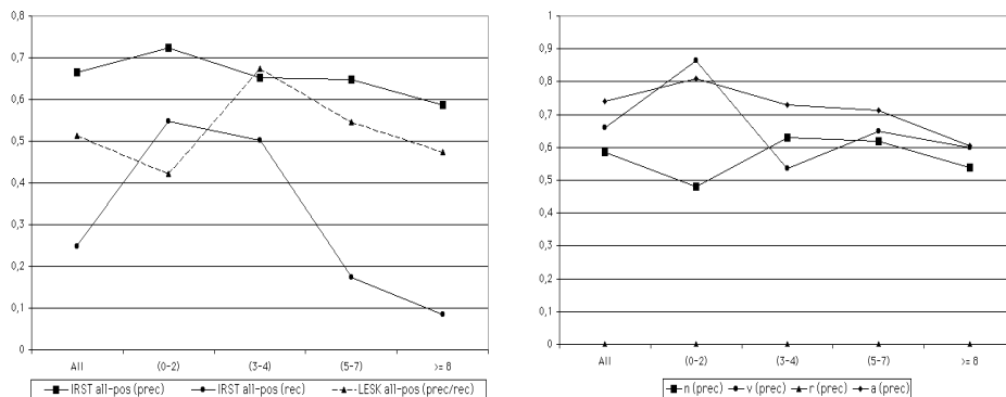
Fig. 5. Lexical_sample Task . On the left a comparison of our system with the “Lesk” baseline. On the right the precision of our system for each POS.
