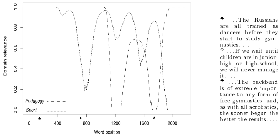
Fig. 2. Domain variation in the text br-e24 from the Semcor corpus.
