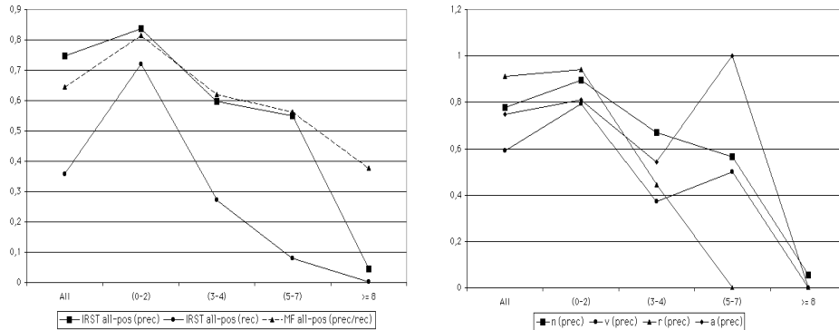
Fig. 4. All_words Task . On the left a comparison of our system with the “most frequent” (MF) baseline. On the right the precision of our system for each POS.
